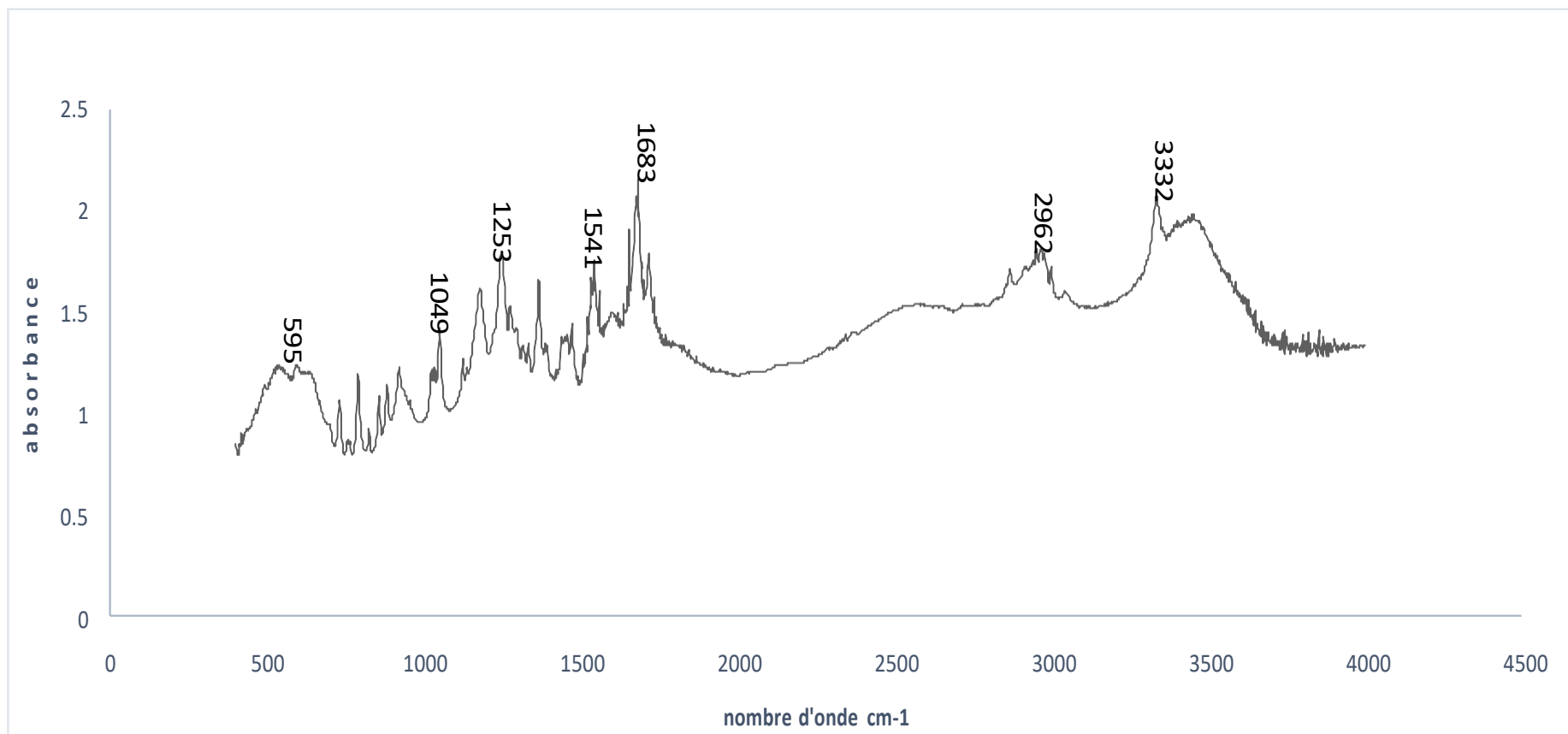
Figure 53 : Spectre FTIR du Boc-Leu-OH
