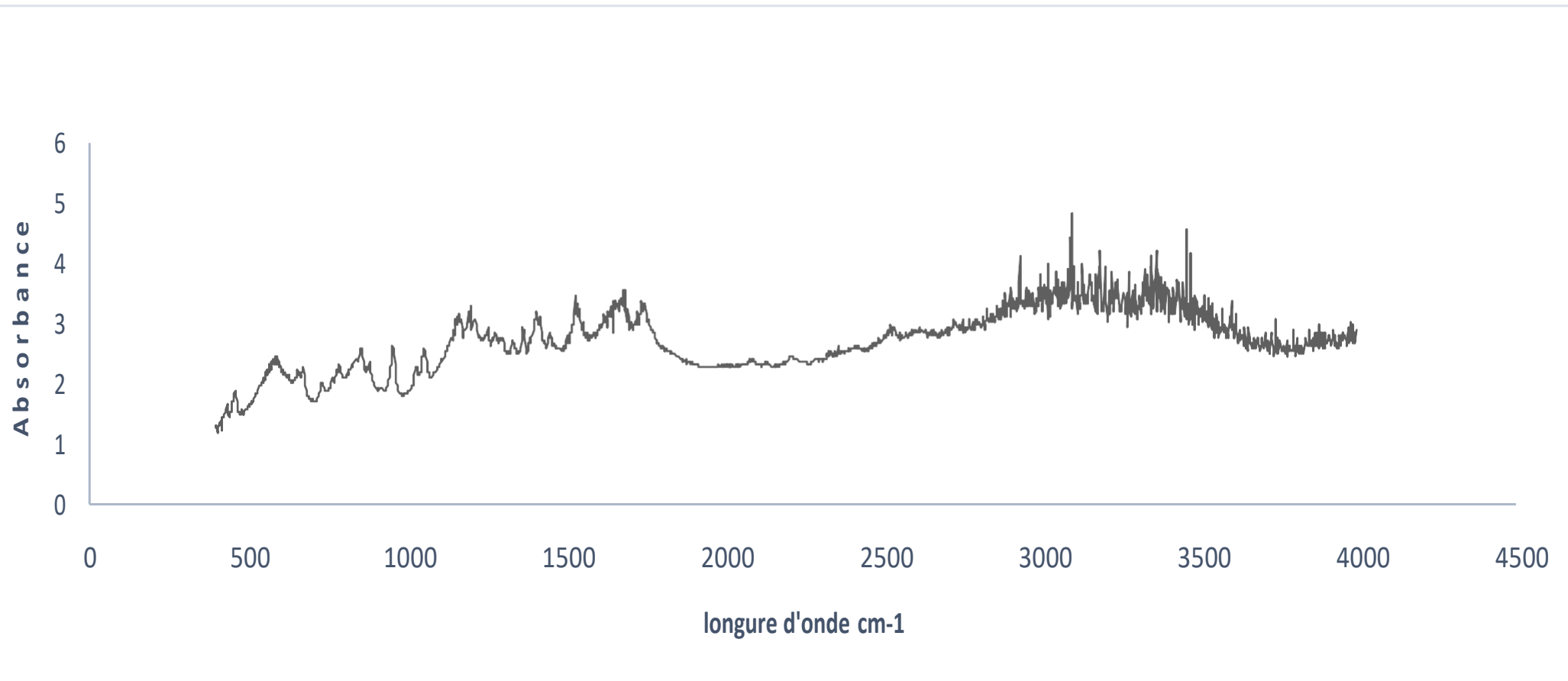
Figure 49 : Spectre FTIR du Boc-Gly-OH.
