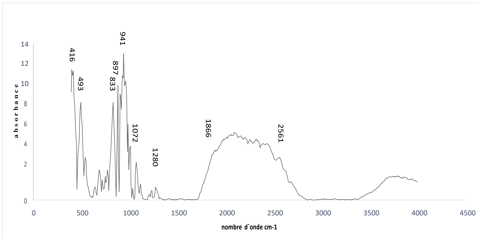
Figure 48 : Spectre FTIR du Boc-Gly-NHiPr.
