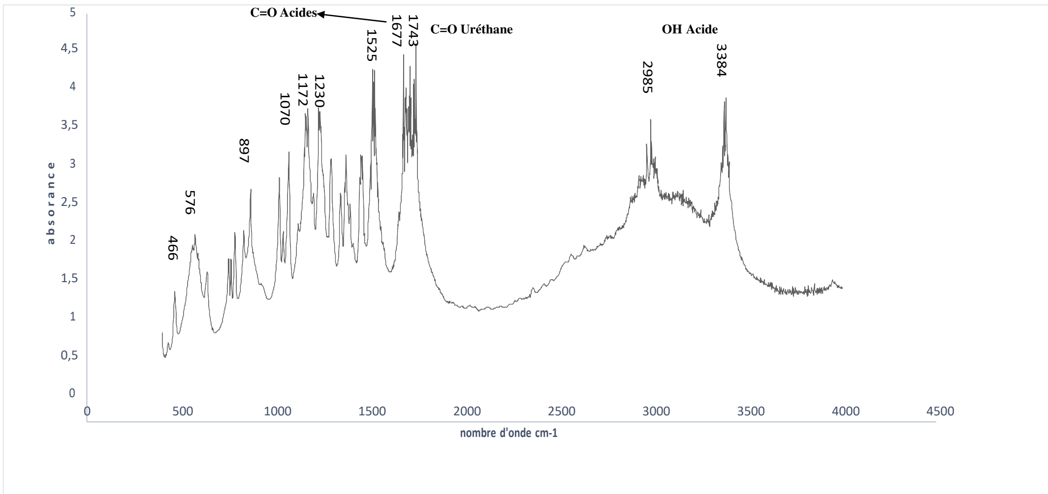
Figure 44 : Spectre FTIR du Boc-Ala-OH.
