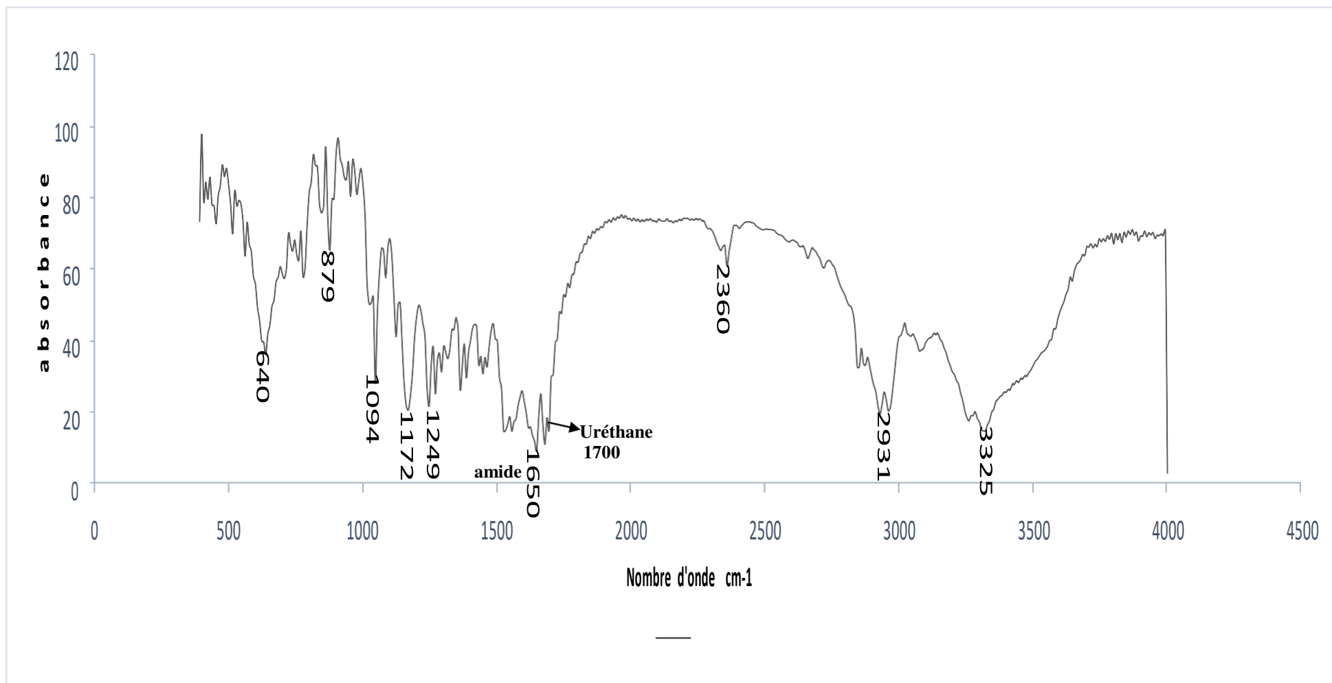
Figure 52: Spectre FTIR du Boc-Leu-NHiPr
