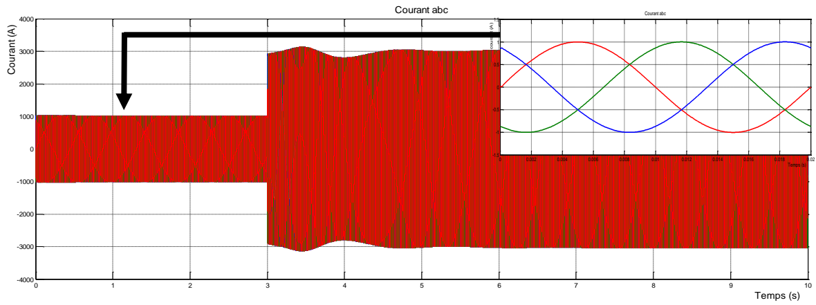
Figure III.14 :courant abc de la machine synchrone
