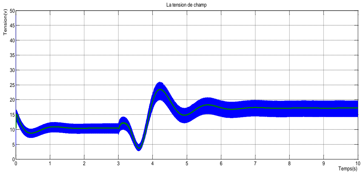
Figure III.9 :La tension de champ.
