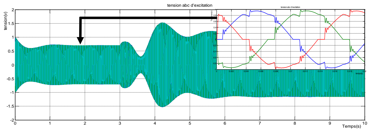
Figure III.15 :tension abc d'excitation
