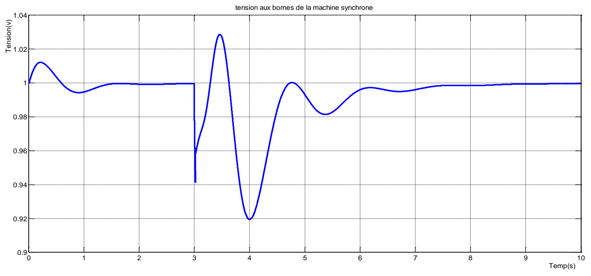
Figure III.10 : Tension aux bornes de la machine synchrone.
