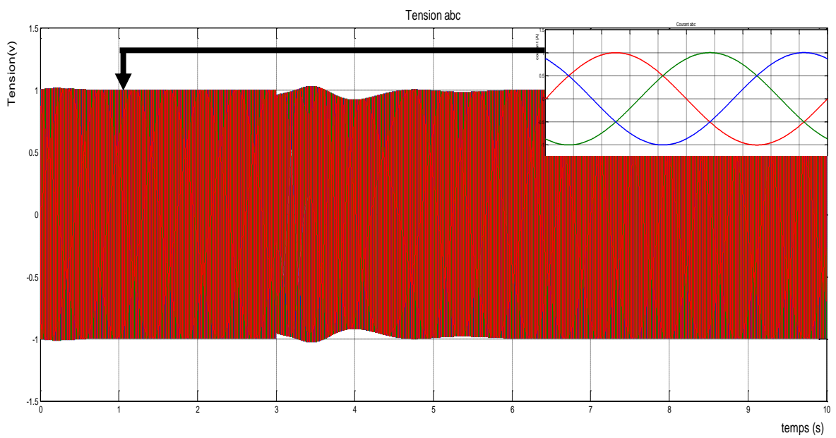
Figure III.13 : tension abc de la machine synchrone
