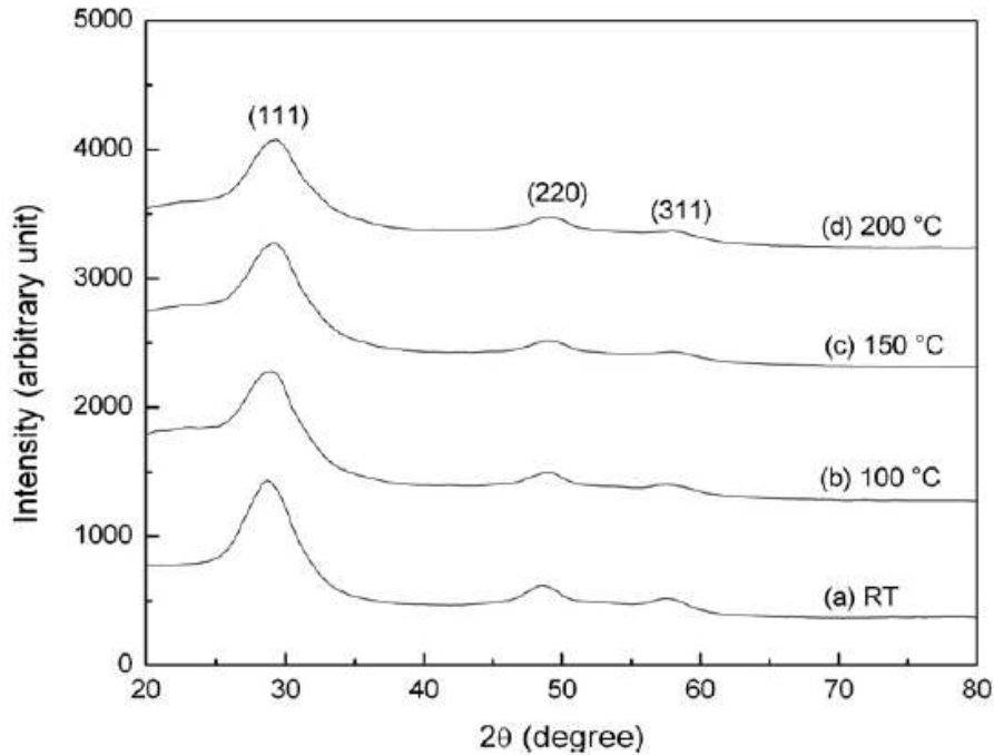
Figure I. 12: XRD patterns of the deposited ZnS thin films at different annealing temperatures [63].
