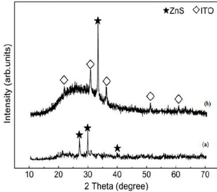
Figure I. 3: XRD patterns of the film (a) before and (b) after annealing [14].
