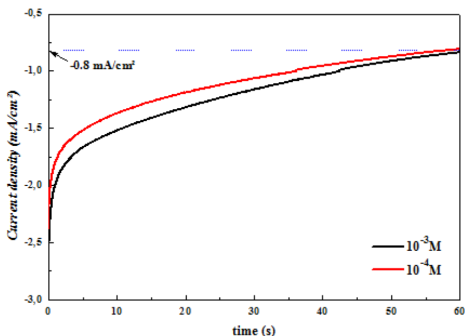
Figure III. 3: Experimental current transients of the electrodeposited ZnS on ITO at two concentration of \text{ZnSO}_4 .
