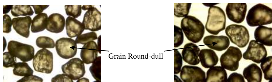
Morphoscopy of the quartz grains for the samples in the Algerian Bas-Sahara (Fraction 500-315 \mu\text{m} )
