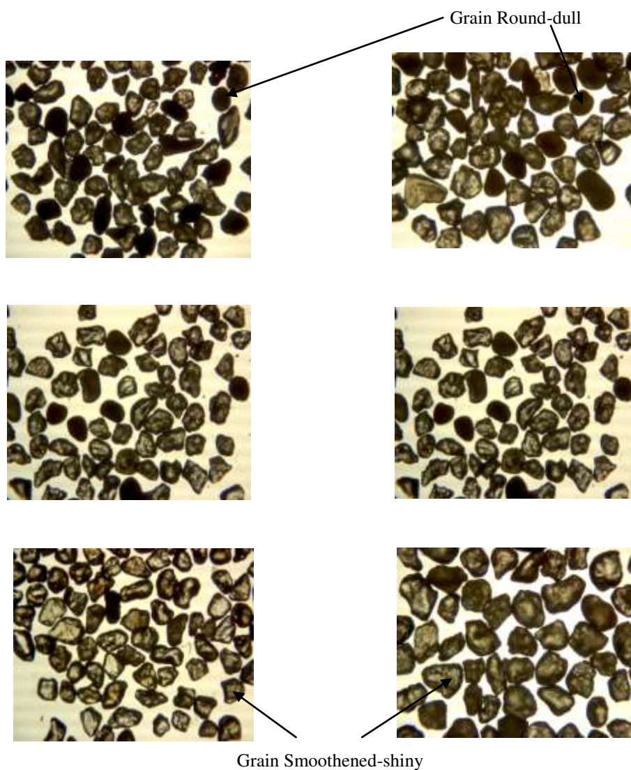
Morphoscopy of the quartz grains for the samples in the Algerian Bas-Sahara (Fraction 315-200 \mu\text{m} )
